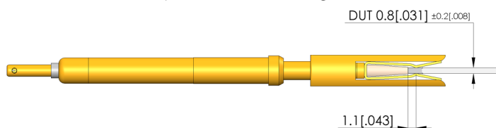
Example of contact at working stroke
