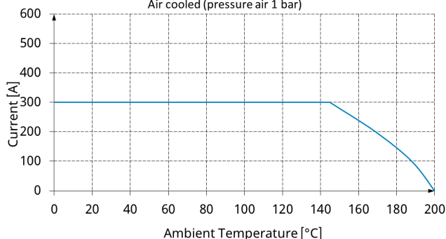
Current Derating
